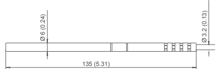
HMT337 T probe
